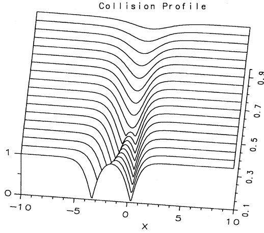
Figure 4. Profile of the collision pattern of two ideal dark solitons as a function of \zeta . Note that for \zeta < 1/2 , the collision profile possesses two dips.
