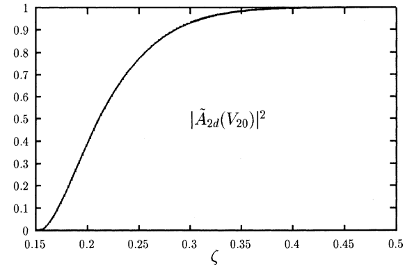
Figure 7. Intensity of the k_x = V_{20} component of the diffracted probe beam as a function of \zeta . Here, h = 1/2\zeta and \beta = 2 .
