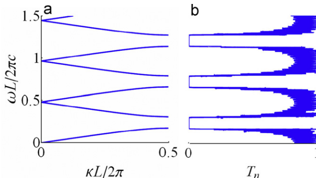
Fig. 3. For the DPC substrate \delta = 0 : (a) the band structure; (b) the stopgap for 10 periods. In both pictures a = 0.1082 \mu\text{m} , b = 0.2654 \mu\text{m} and n_1 = 3.58 and n_2 = 1.46 .
