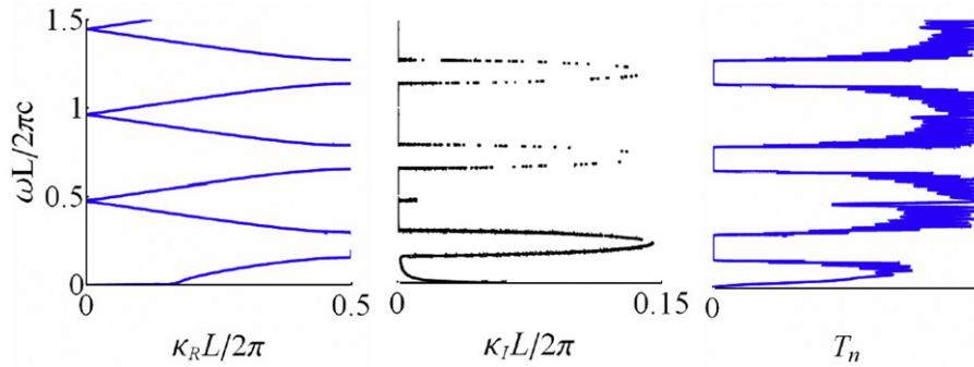
Fig. 4. The stopgap, band structure and the absorption for a MDPC for the same parameters that in Fig. 3, in this case \delta = 0.001 \mu\text{m} .
