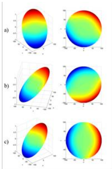
Fig. 3. Same as Fig. 2 but for Seidel primary coma.
