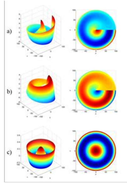
Fig. 2. The generation of Zernike's spherical aberration.
