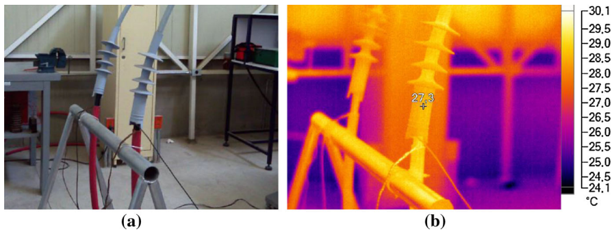
Fig. 10 Pictures of the terminal in good condition in two different color palettes: (a) white light and (b) infrared
