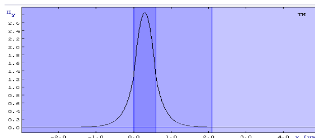
Figure 2 Numerical determination of PDLC thickness on a Si substrate.
